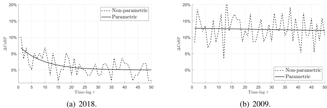
FIGURE 1. Illustration of \Delta\text{CoSP} Dynamics.
