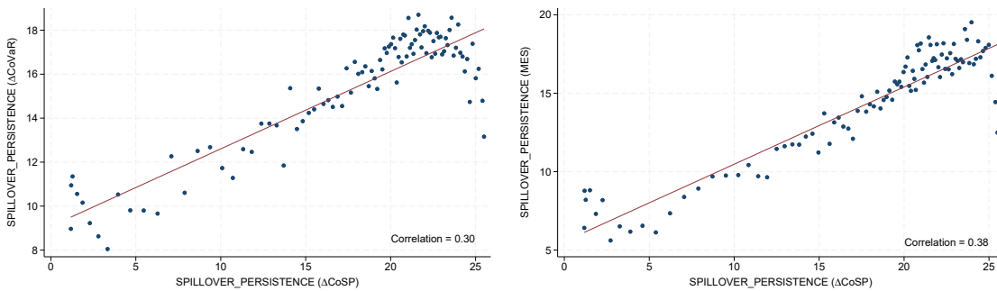
(a) \Delta\text{CoSP} and \Delta\text{CoVaR} .
