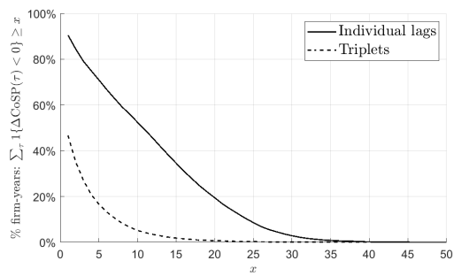
(b) Observations with Negative \Delta\text{CoSP}_\tau .
