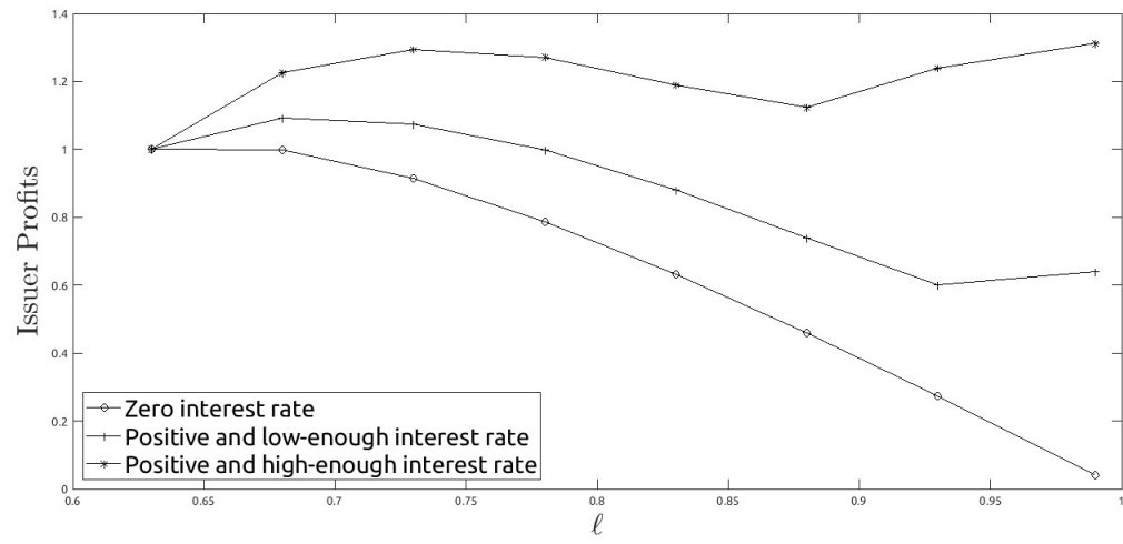
Figure A.5: Stablecoin issuer's profit for different l and r .
